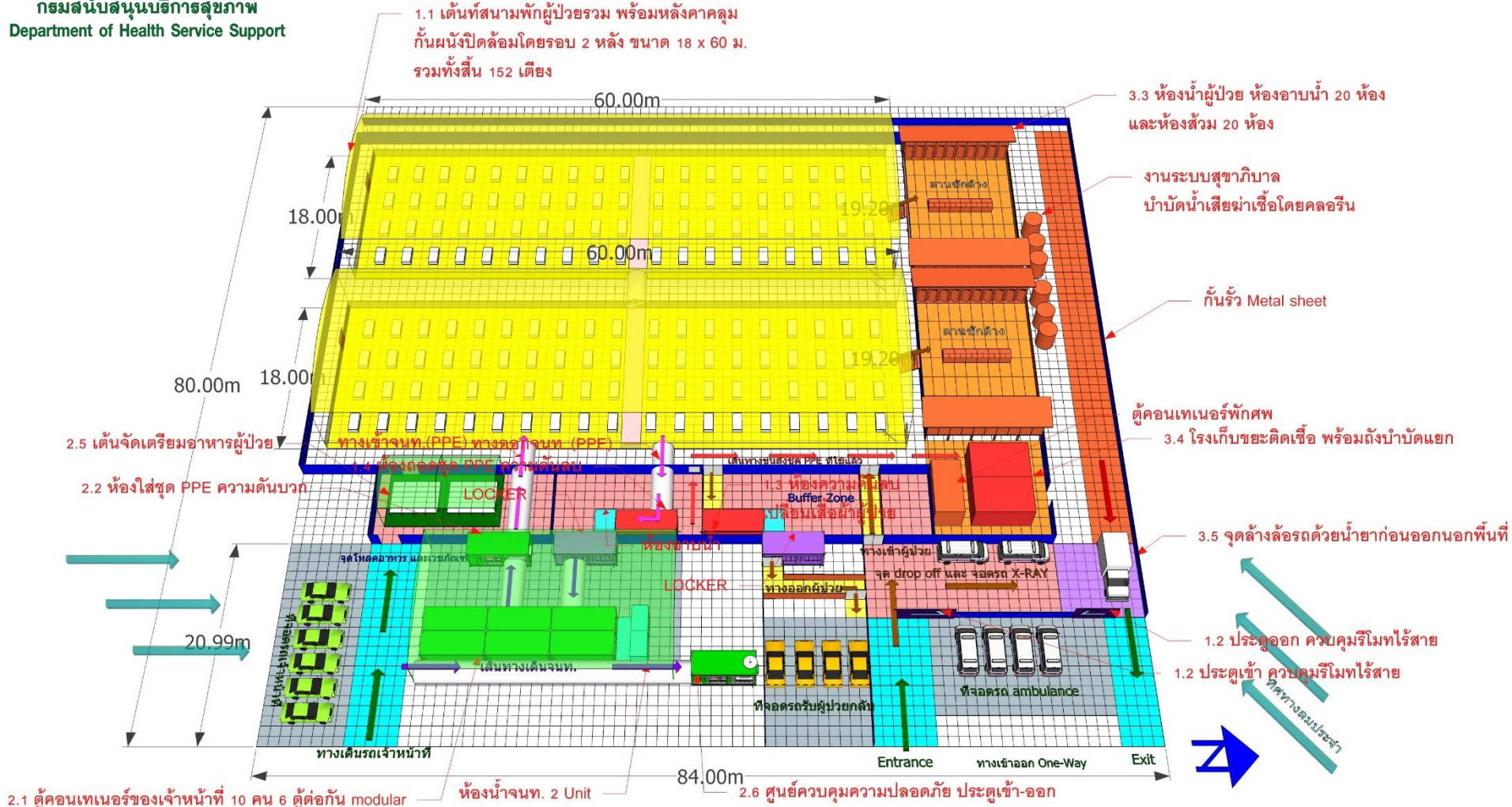
Master Plan Field Hospital 150 Bed
